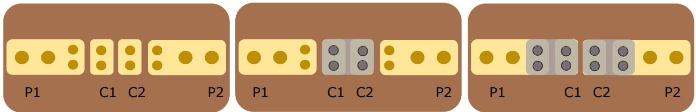
Figure 3: Current transformer (medium voltage block design) with switching capability
